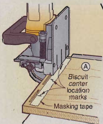
DRAWING 1 Cutting biscuit slots near the ends of the sides
